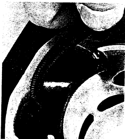
Hard-edged transfer port dividers can be rounded nicely with the inside surface of a hooked file.
