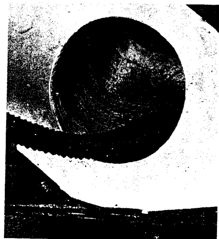
A bent, coarse-toothed rasp is being used here to round a sharply-angled intake port entry.
