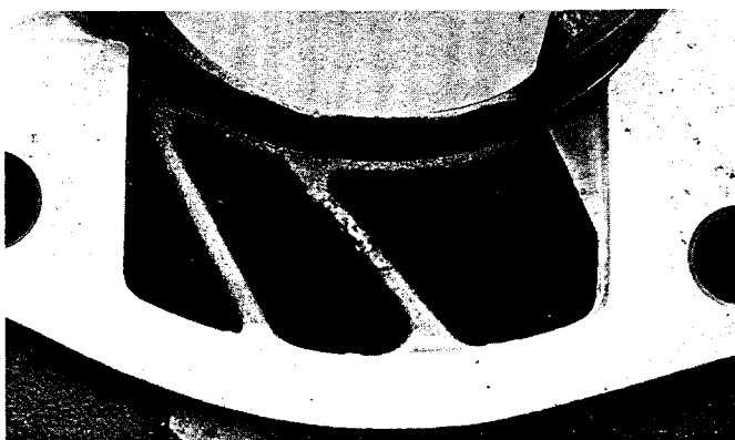
Roughness around the transfer entry tends to block flow up into the cylinder.
