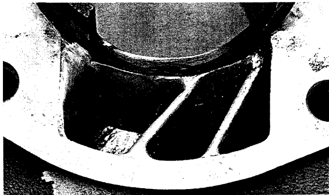
Work inside the transfer tunnels is most difficult, but also most effective.
