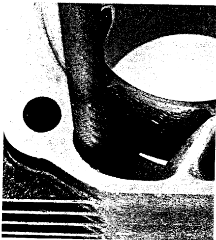
The hooked tip of a reworked rat tail file will reach the important transfer port outlet area.
