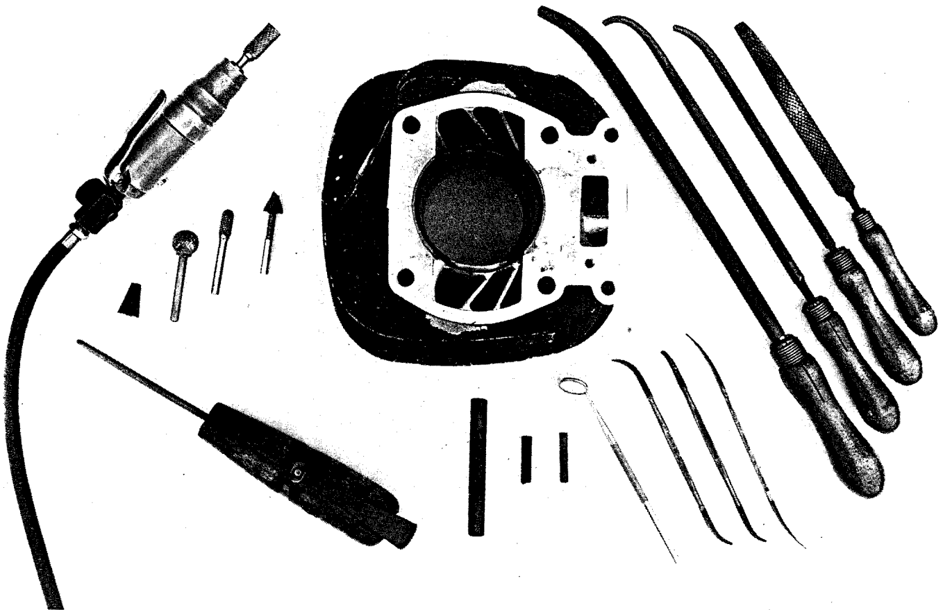
We used an air motor and rotary files to speed some of our clean-up work; it can all be done with ordinary rat-tails, rifflers and fine-grit stones.
