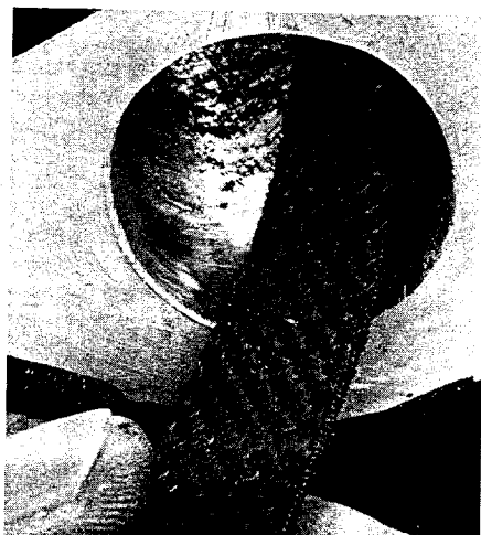
Flow-improving pockets and arches can be carved in ports with a suitably curved half-round rasp.
