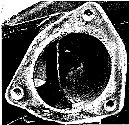
It's especially important that an exhaust port's walls be smooth, but don't thin the bridge.
