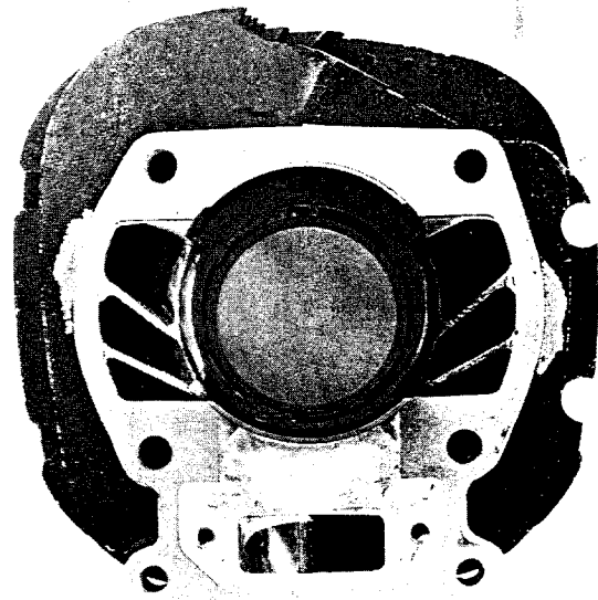
This cylinder's left side has been reworked lightly for improved air flow through its numerous ports.
