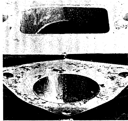
You can remove enough metal to match port/manifold edges; changing port shapes asks for trouble.
