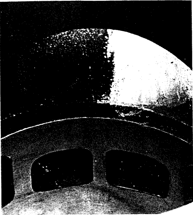
After the port clean-up and re-boring, the port window edges are rounded off.
